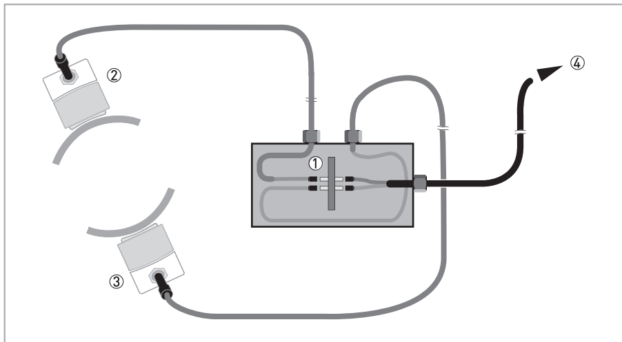
Figure 4-12: Example of large sensor rail connections with cable (splitter) box
