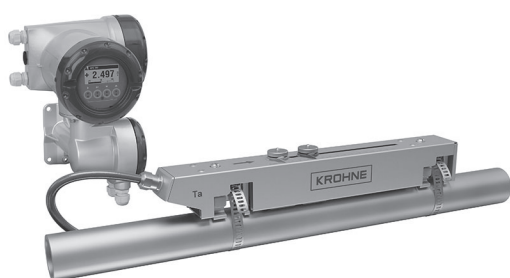
Figure 1-1: OPTISONIC 6000 Small rail with UFC 300 F
