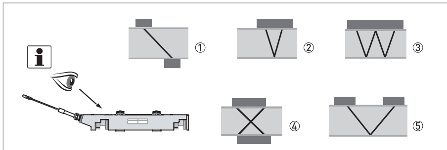
Figure 3-10: Measuring modes
